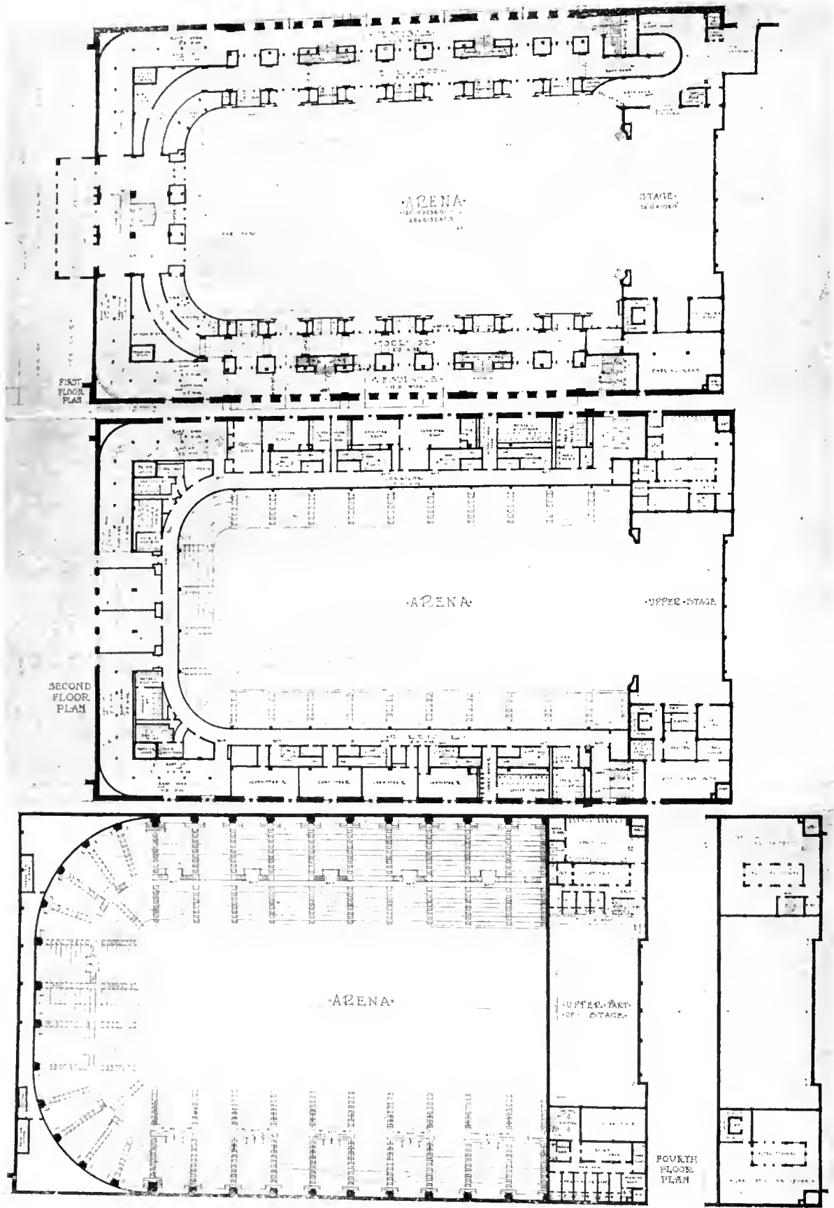
FLOOR PLANS OF THE CLEVELAND AUDITORIUM J. H. MACDOWELL, ARCHITECT. F. R. WALKER, CONSULTING ARCHITECT
